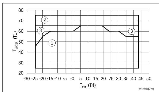
8. ábra CS2000AWF 4-6 R-S, CS2000AWF 8-10 R-S, CS2000AWF 12-16 R-S/T
